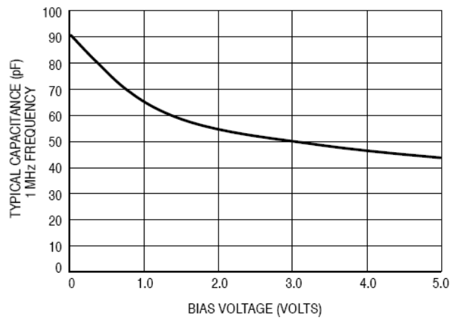
Figure 4. Capacitance
